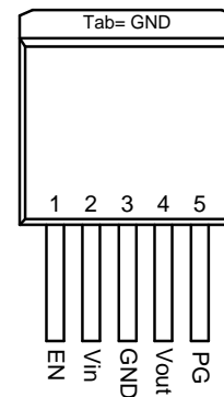
TO263-5 (Top View)
