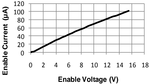
Enable Current vs. Enable Voltage
